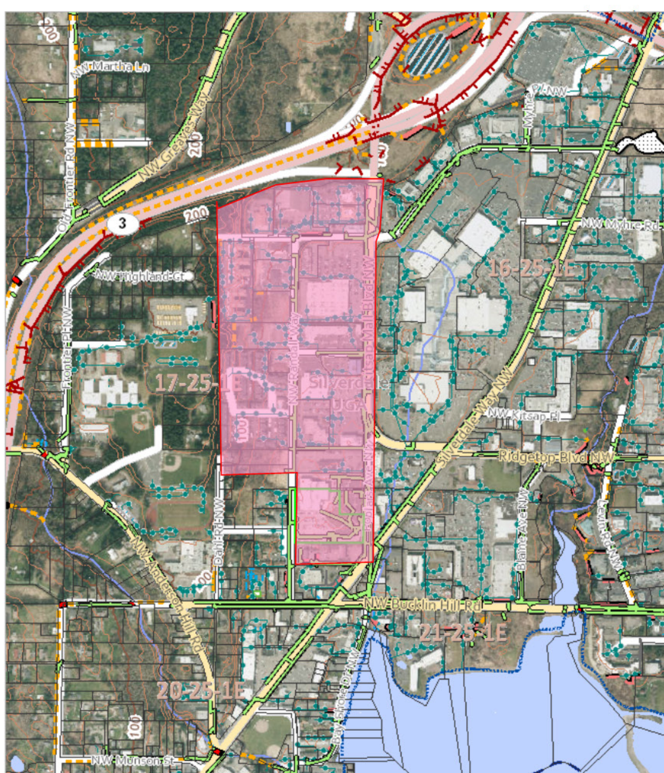
UPSTREAM STORM WATER BASIN MAP ~ 90 Acres
